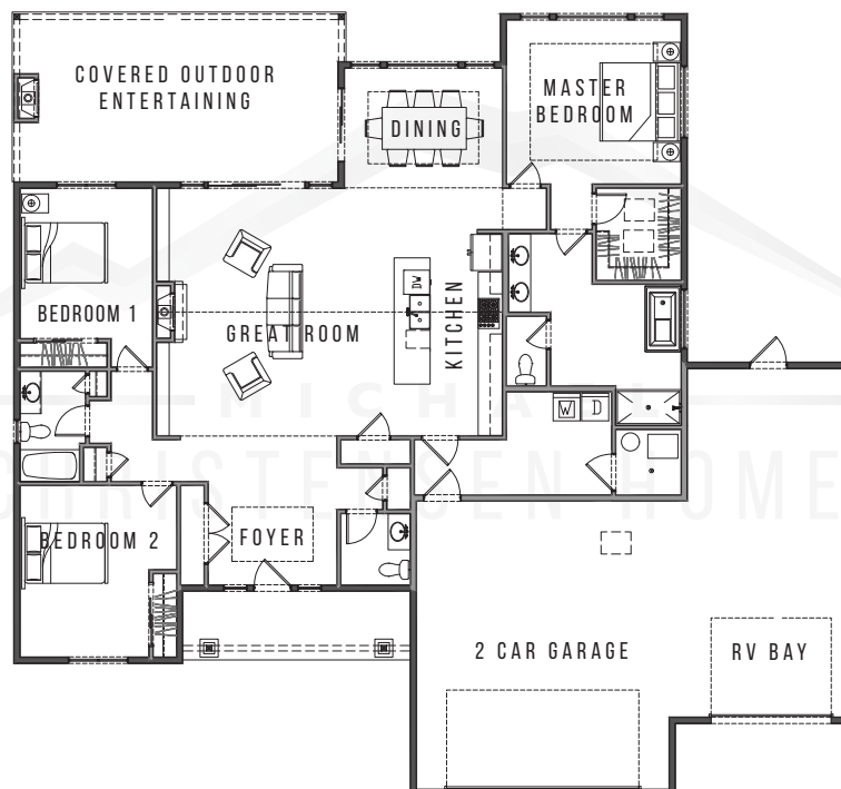
MAIN LEVEL
